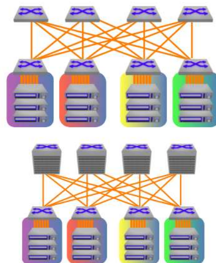
Arista Fixed System Leaf-Spine Designs Scale to 6,144 10GbE/25GbE ports or 1,536 40GbE/100GbE port at 3:1 subscription
