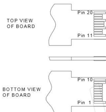
Figure 3, Pin View
