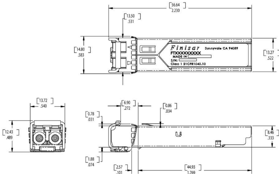
FTLF1319P1BTL
