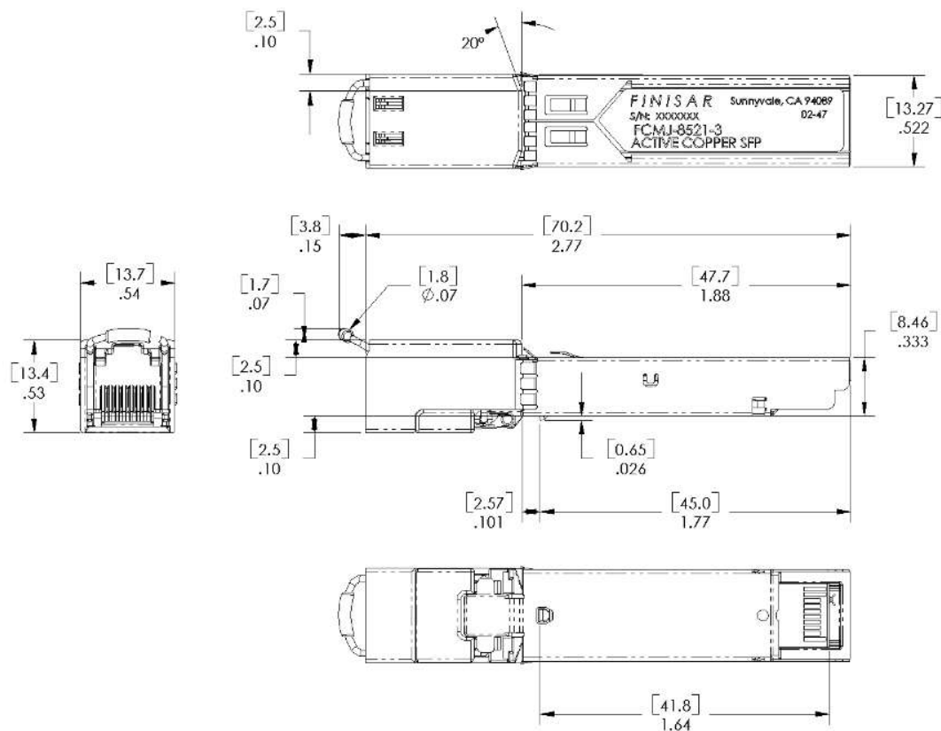
Figure 2. FCMJ-8520/8521-3 mechanical dimensions
