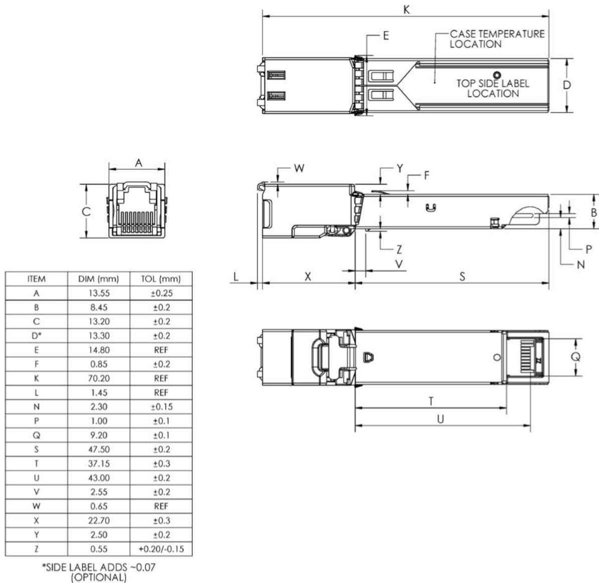
Figure 2. FCLF8520P2BTL, FCLF8521P2BTL and FCLF8522P2BTL mechanical dimensions
