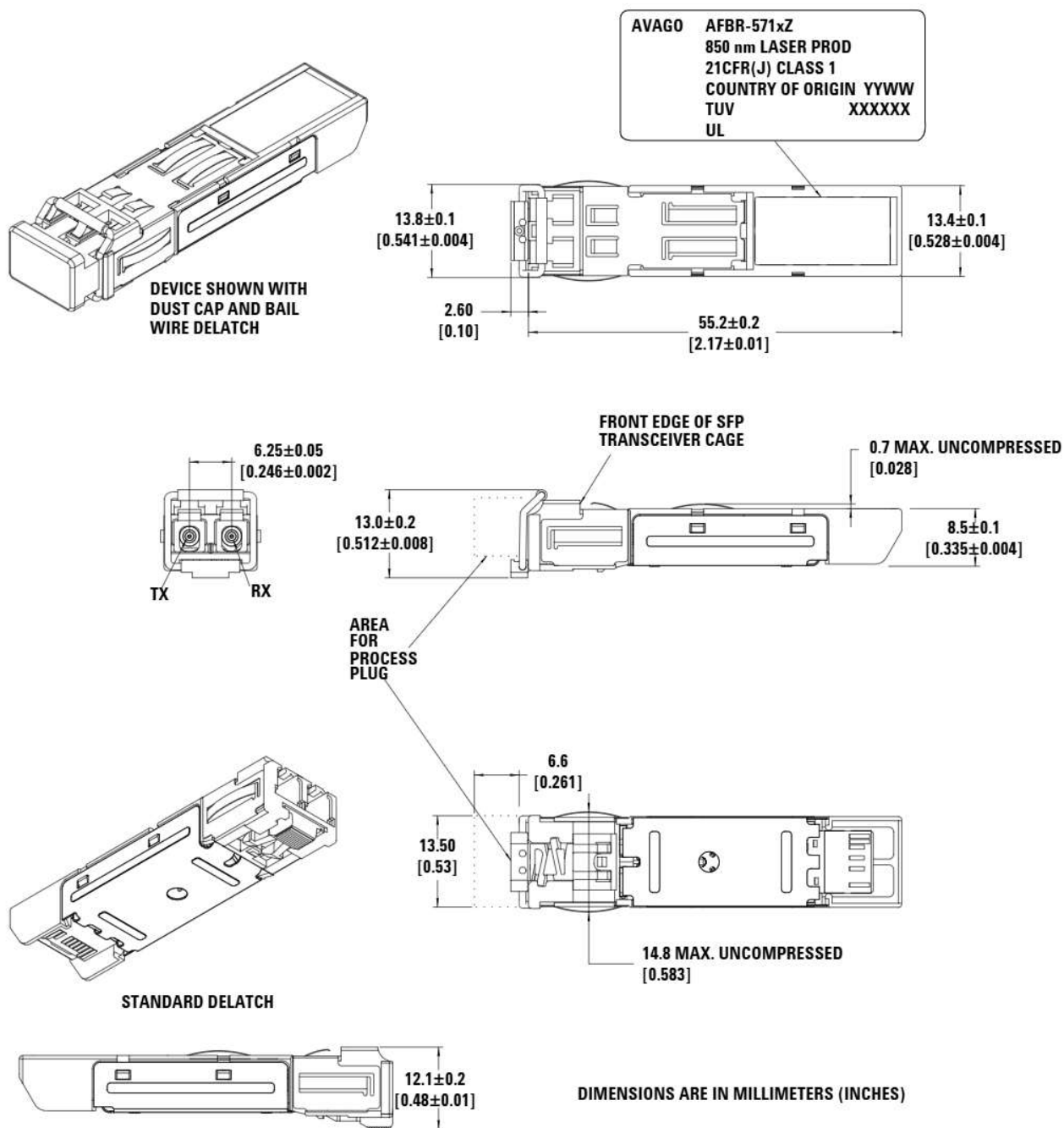
Figure 7. Module drawing
