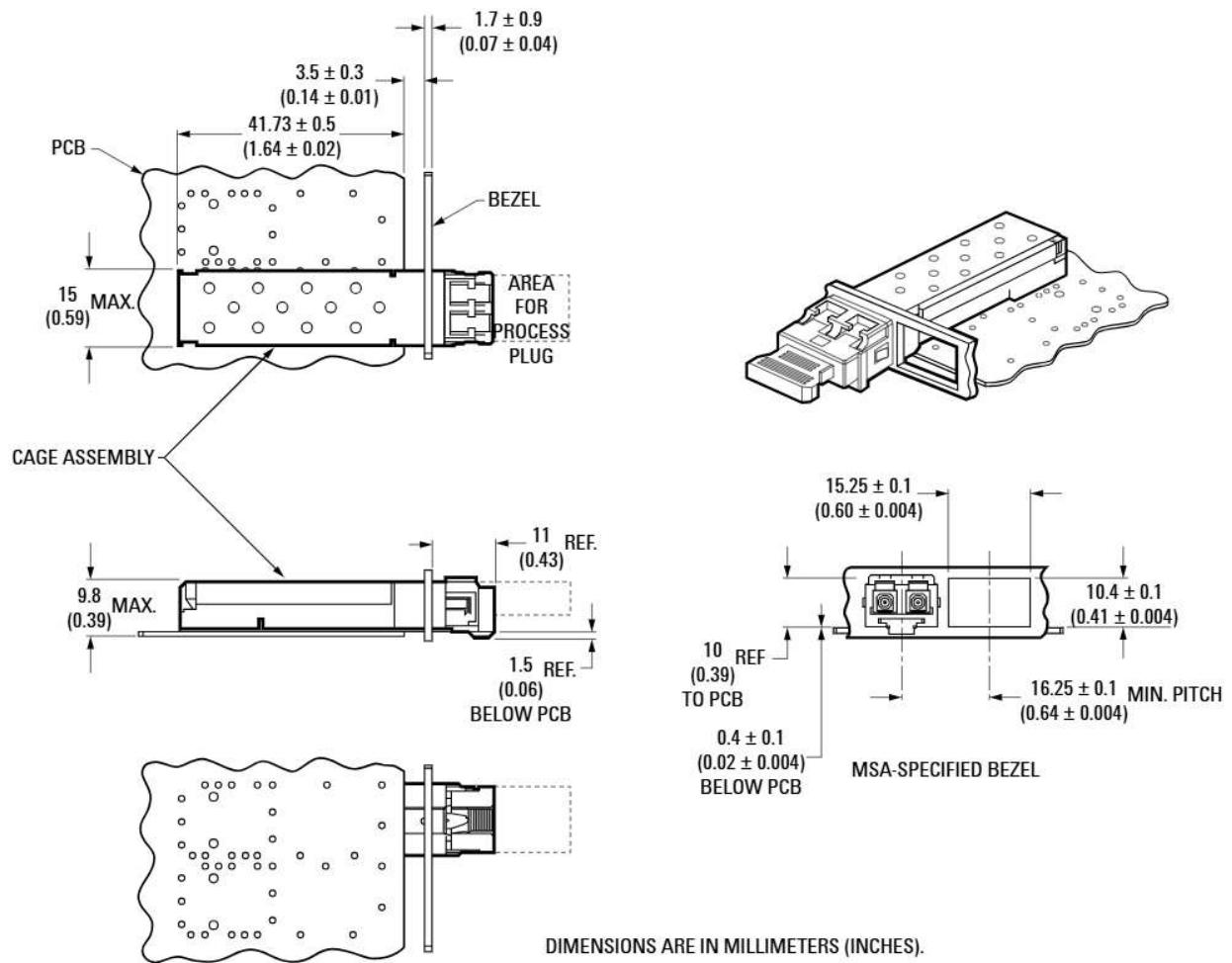
Figure 9. Assembly drawing.
