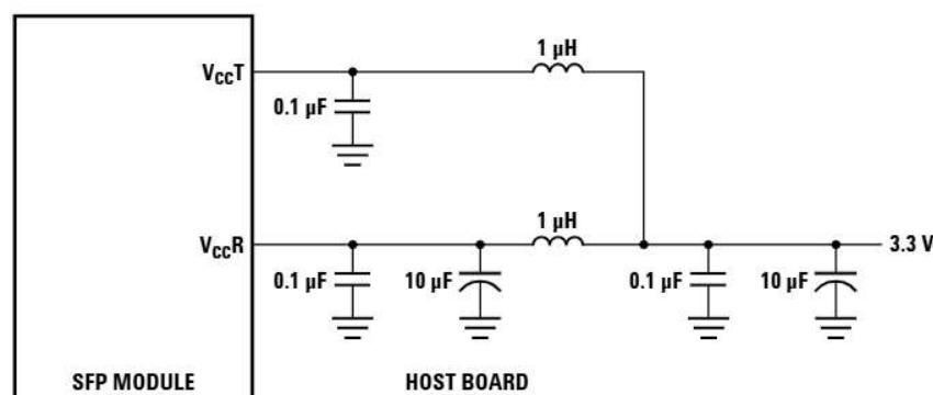
Figure 4. MSA required power supply filter.
