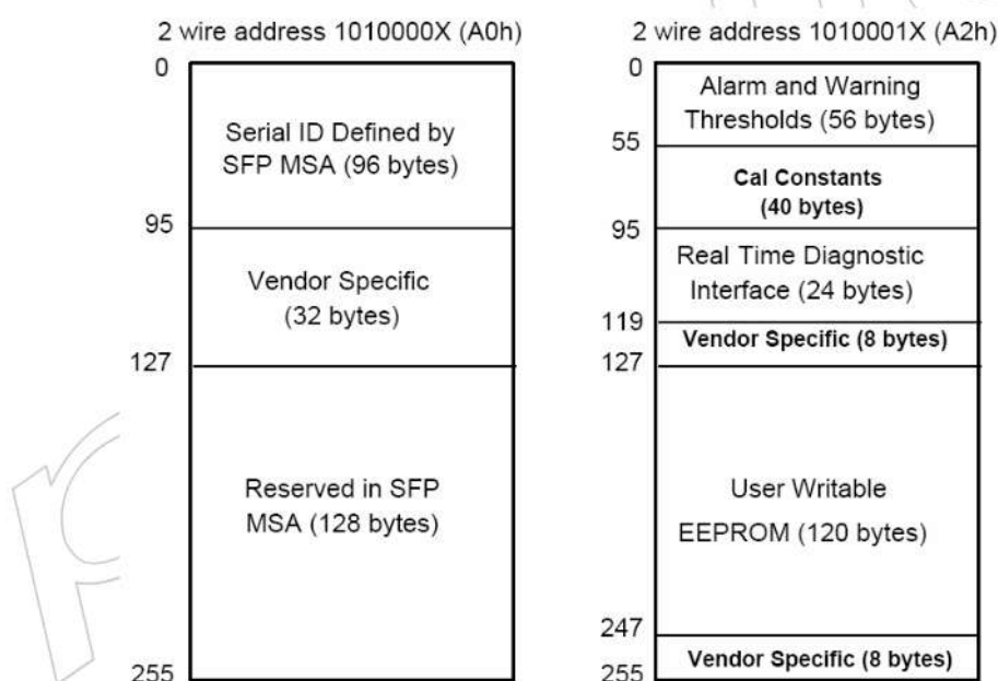
Figure 1, EEPROM Memory Map Specific Data Field Description
