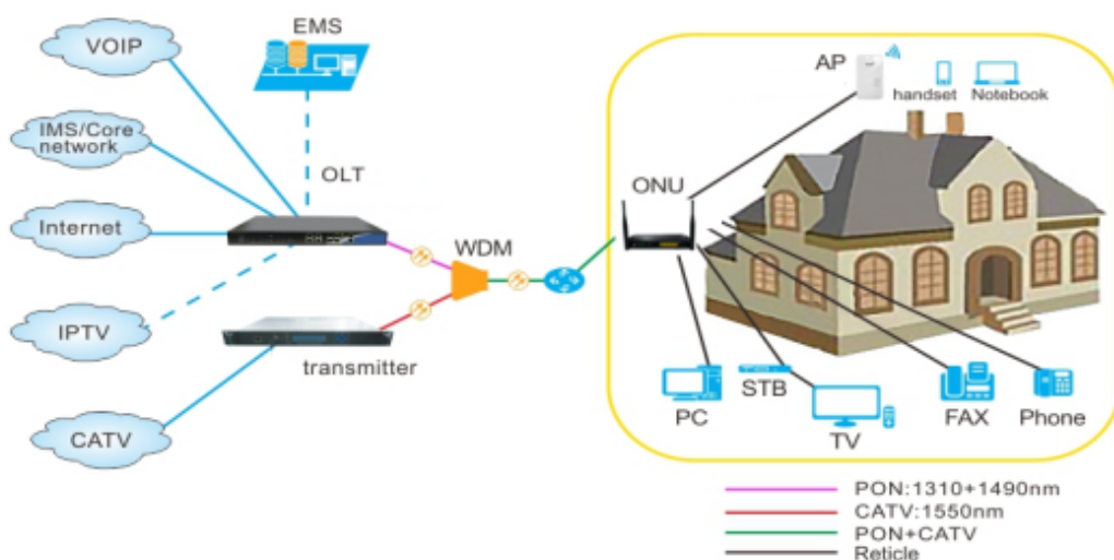
Picture 1-1 RH841GWVC-AX3B Products Network diagram
