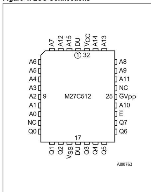
Figure 4. LCC Connections
