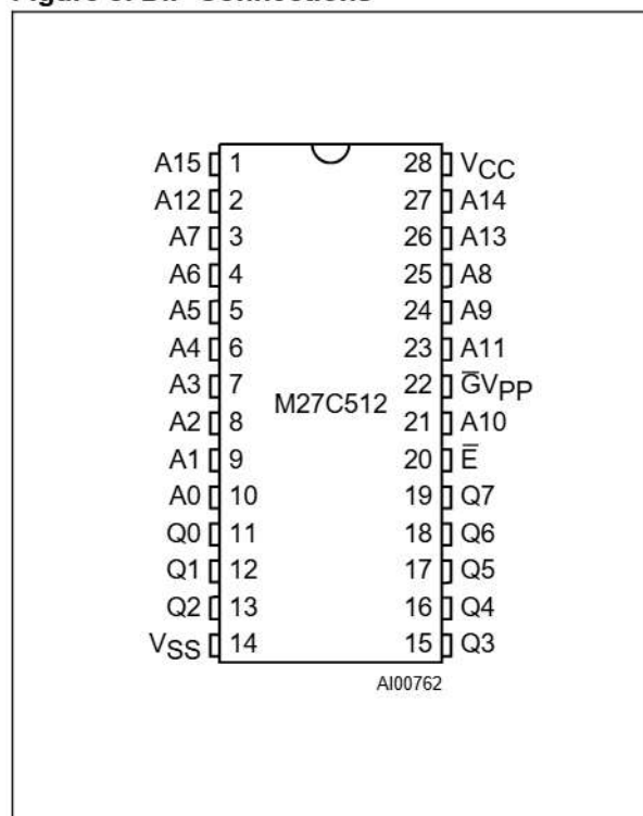
Figure 3. DIP Connections
