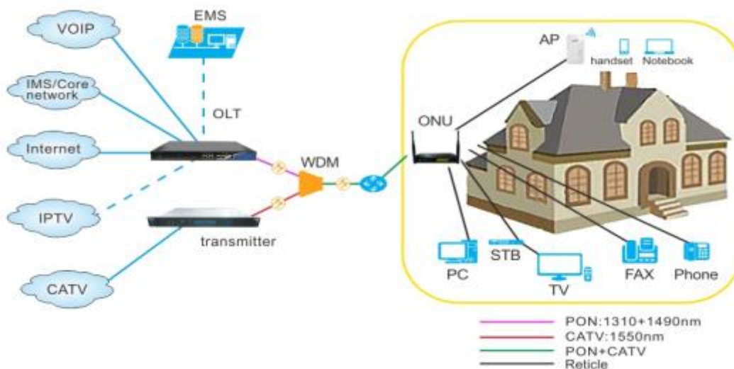
Picture 1-1 RH841GWV-AX3 Products Network diagram
