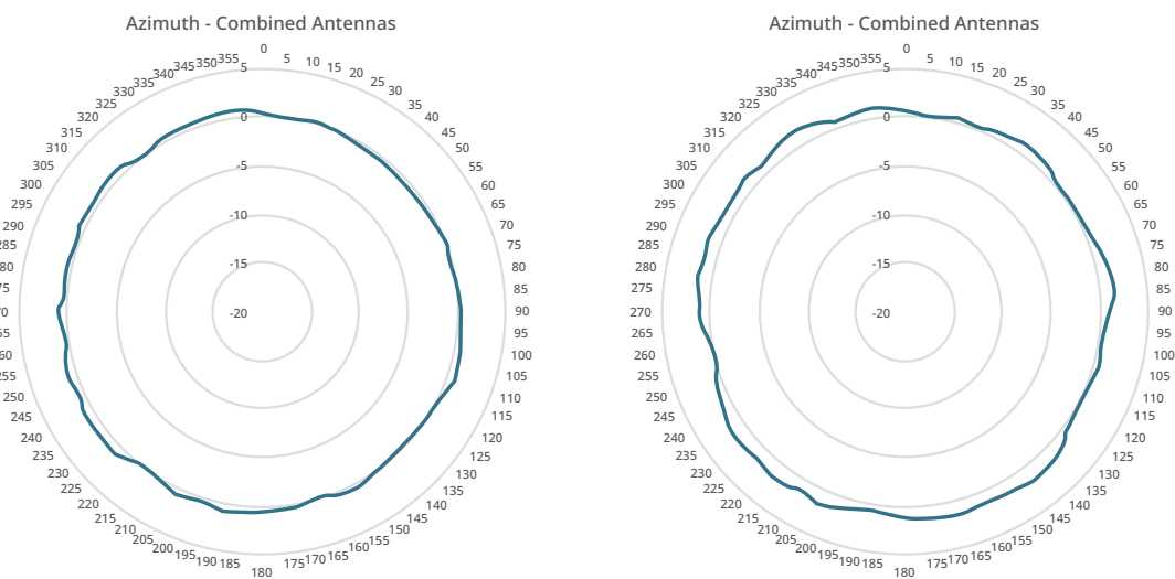
2.4 GHz (Left) and 5 GHz (Right) Azimuth Antenna Patterns
